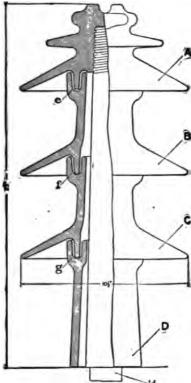
FIG. 12. EXPERIMENTAL HIGH-TENSION INSULATOR.
